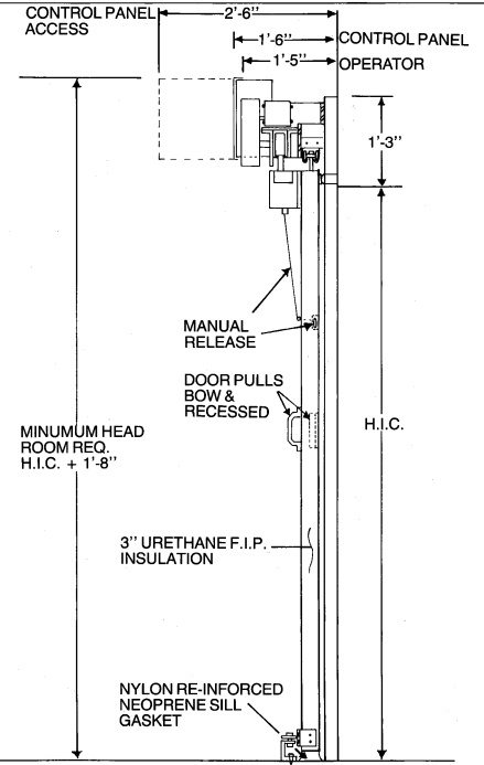
SECTION
