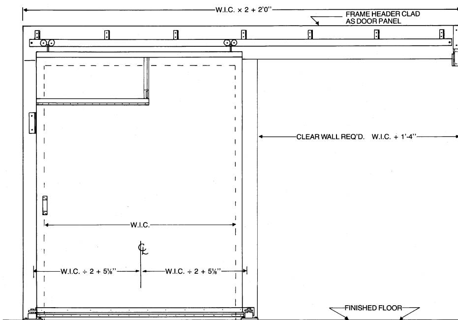
ELEVATION RIGHT SLIDE TO OPEN SHOWN LEFT SLIDE MIRROR IMAGE
