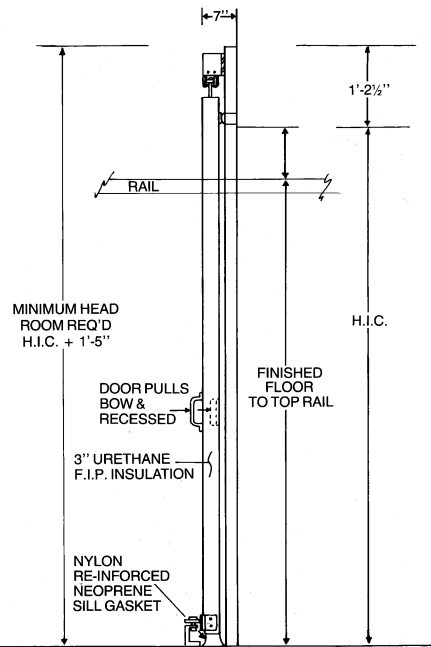
SECTION
